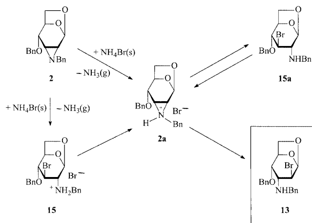
Figure 2. Reaction pathway for the formation of bromo derivative 13
