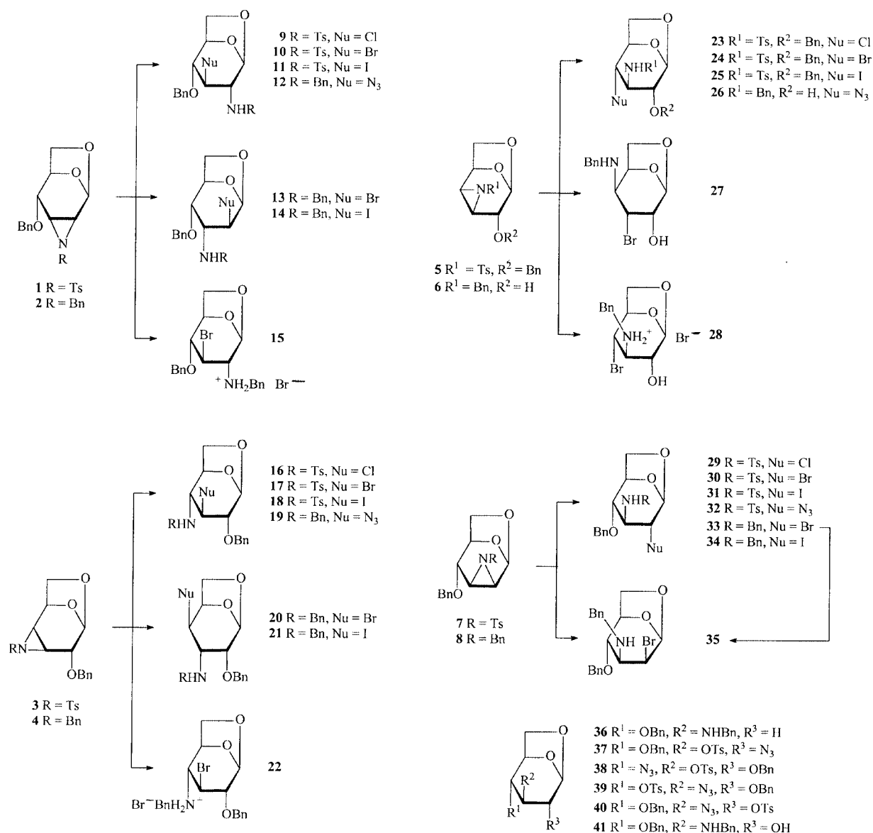
Figure 1. Starting epimines 1–8 and the products 9–41 of the reactions performed
